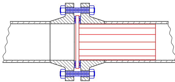
ASSEMBLY
