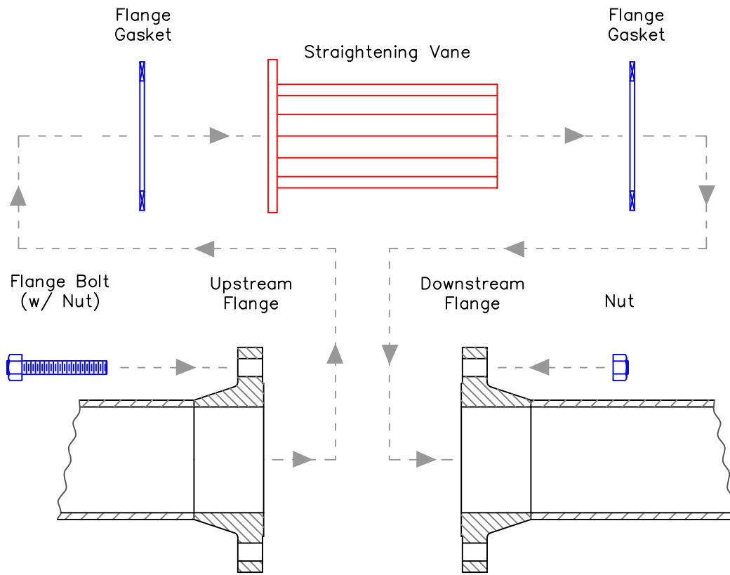
EXPLODED VIEW
