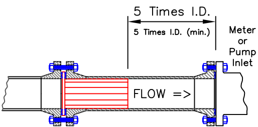
TYPICAL INSTALLATION
