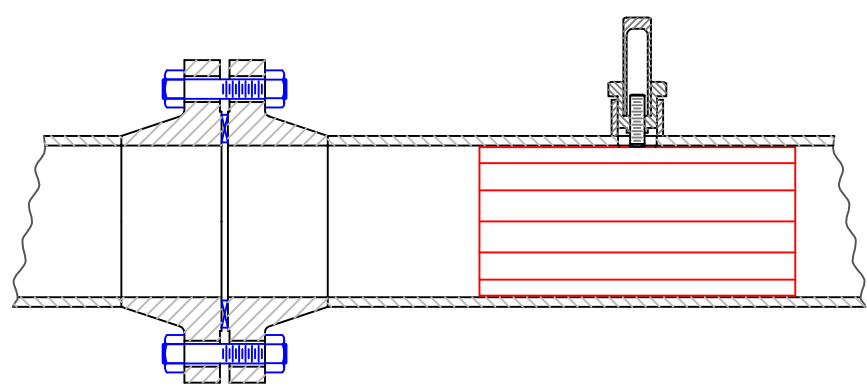
ASSEMBLY
