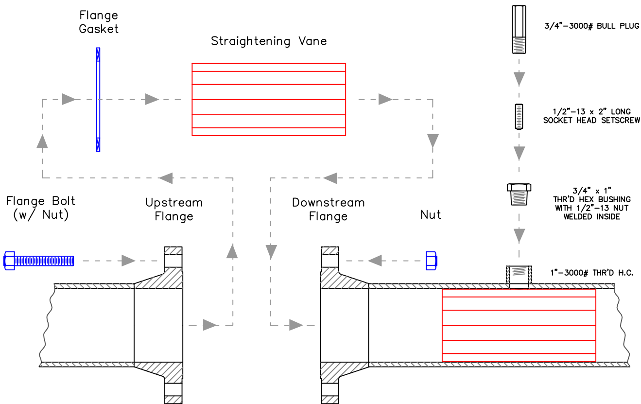
EXPLODED VIEW
